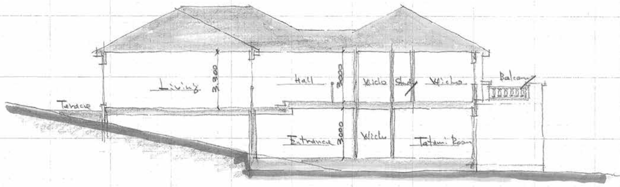
Section 1/100
