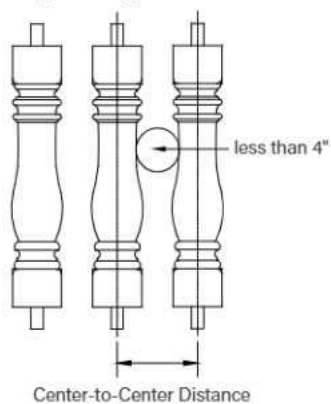
Straight Rail Application
