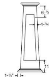
Recess is 1/2" deep and corners are 1/4" rounded.
