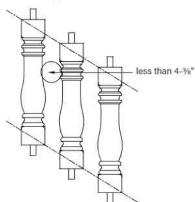
Stair Rail Application
