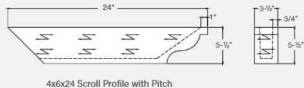
4x6x24 Scroll Profile with Pitch
