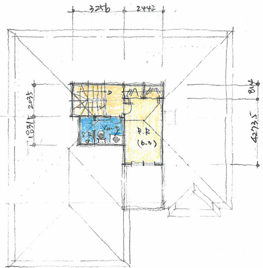
2nd Floor Plan 1/100
