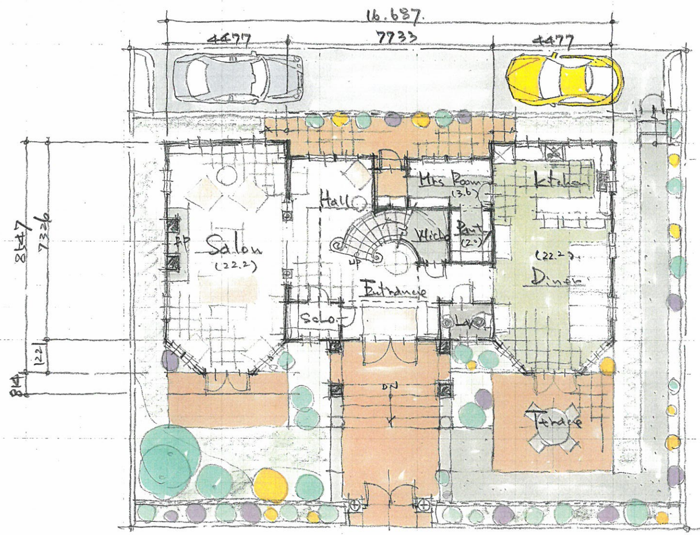
1st Floor Plan 1/100
